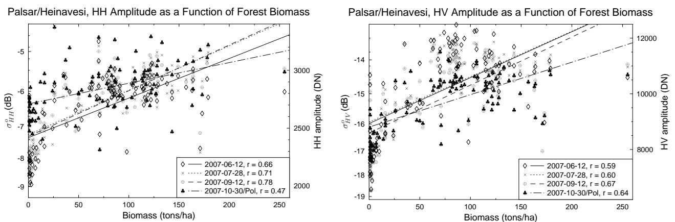
Figure 2. Stand-wise Palsar amplitude data in Heinavesi study site: left HH, right HV.
