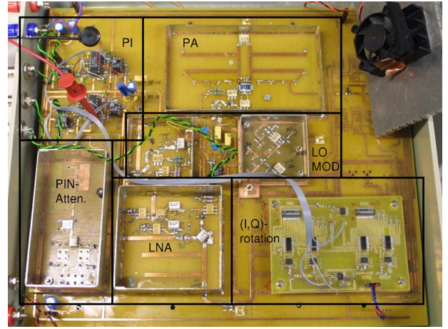
Fig. 3. Photograph of the 865 MHz electronics.
