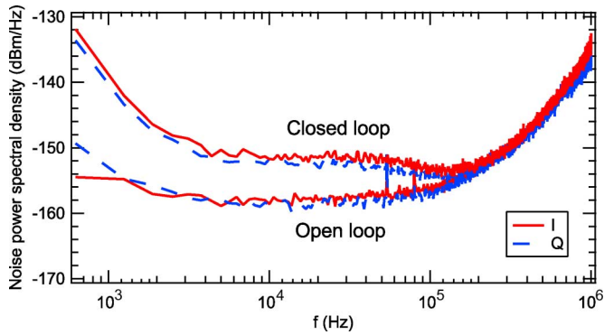
Fig. 5. Measured input referred noise spectral density as a function of offset frequency from the carrier.
