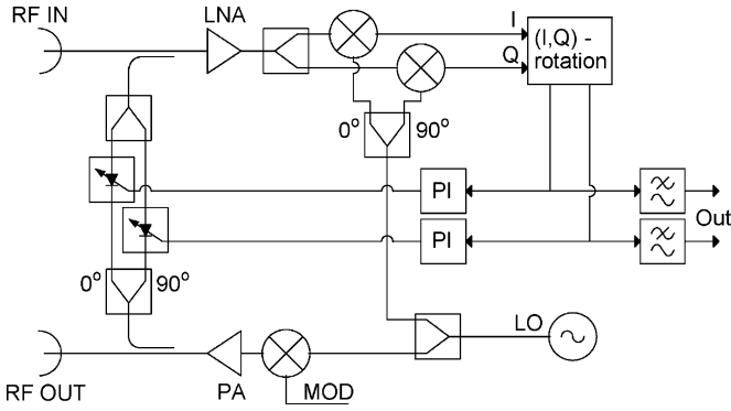
Fig. 2. Block diagram of the reader.
