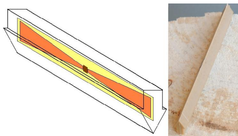
Figure 2. Wedge-shaped transponder
