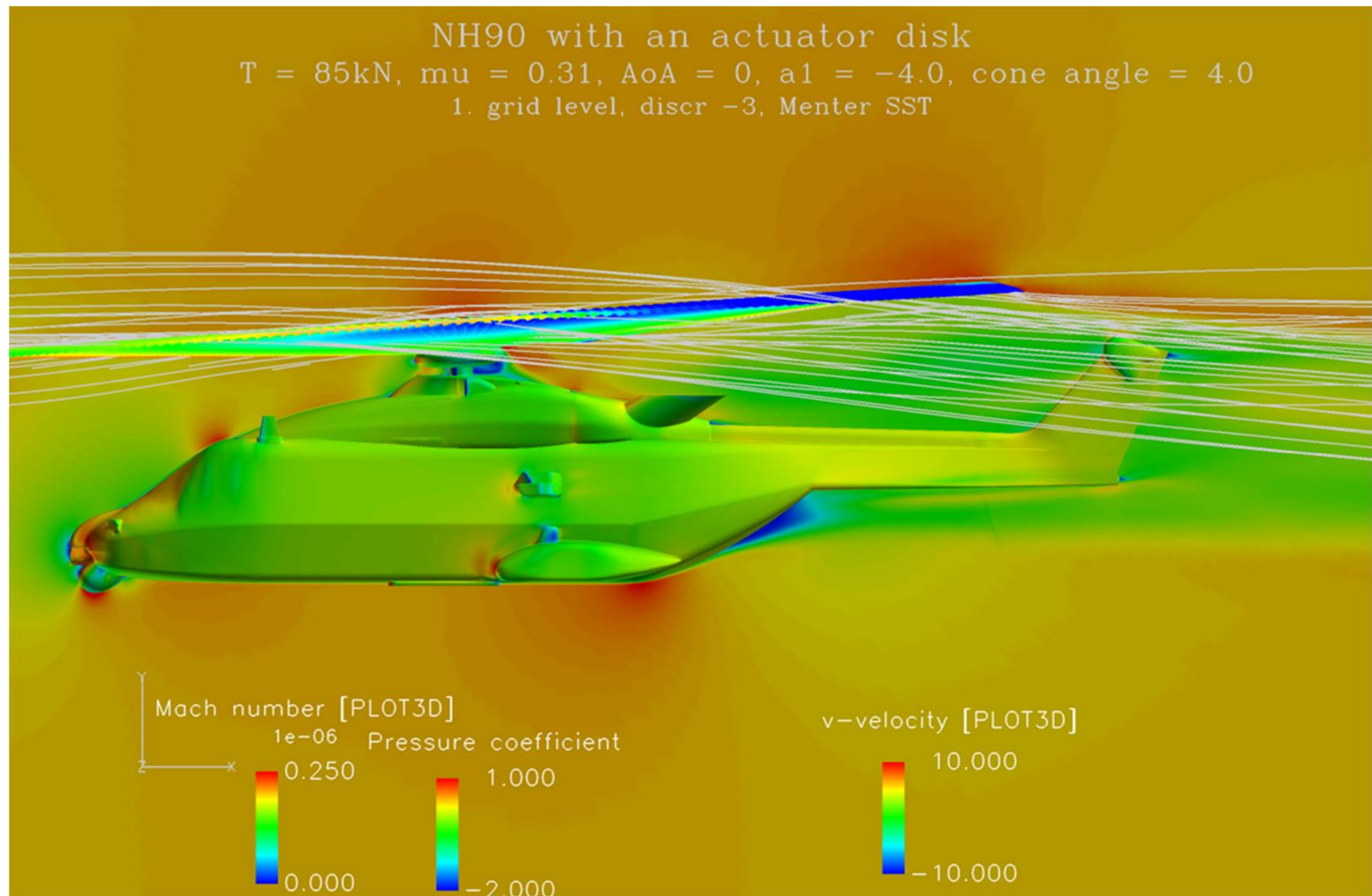
Figure 6: Computed flowfield around NH90 in cruise. Picture by courtesy of Patria Aviation.
