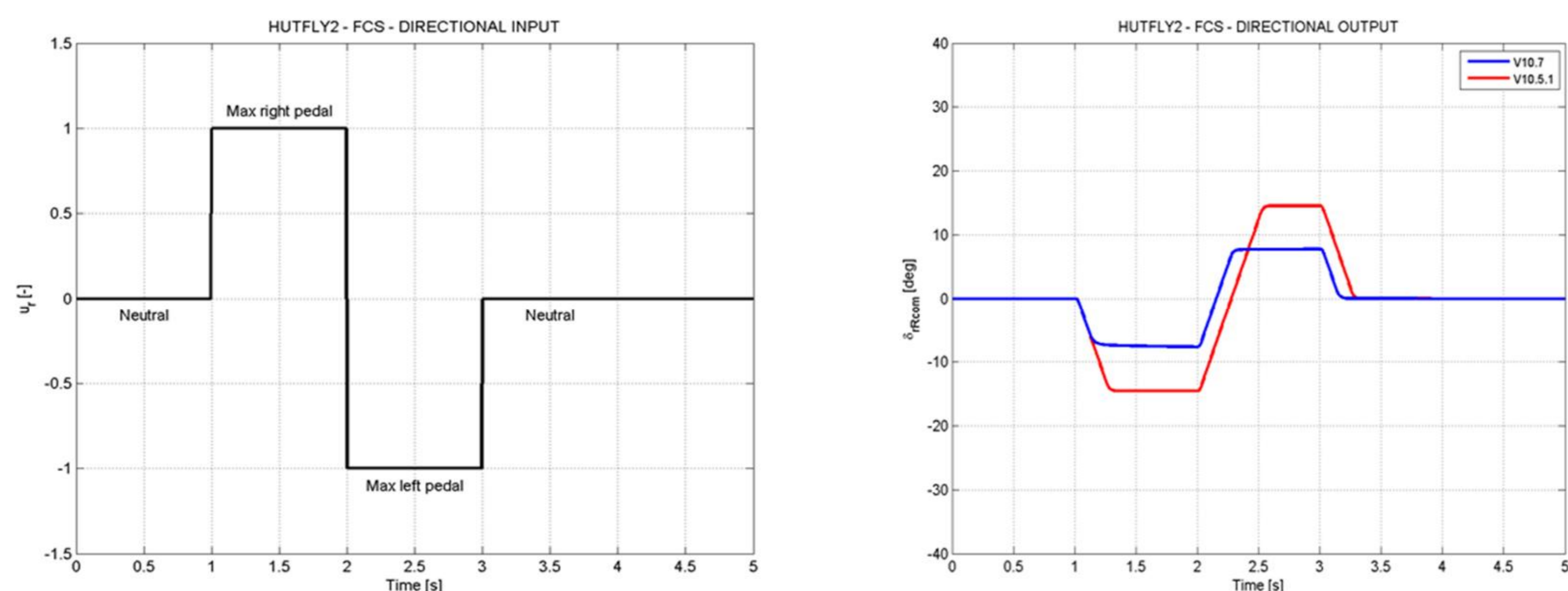
Figure 9: Right rudder actuator command as a response (output; shown right) for the normalized directional control doublet (input, shown left). In output, the red line represents the actuator command from the reference FCS V10.5.1 –model and the blue line represents the command from the upgraded FCS V10.7 –model. Picture by courtesy of VTT.
