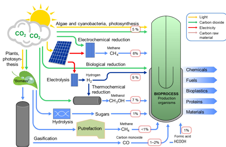
Proposal on the possible routes for carbon dioxide (CO 2 ) conversion into carbon sources suitable for bioprocesses. The percentages indicate the energy efficiency of the conversion in accordance with the first law of thermodynamics (light, electricity and chemical energy were treated equally). The photosynthesis of algae and cyanobacteria produces biomass that may also already contain the desired product. Image: Juha-Pekka Pitkänen & Peter Blomberg
