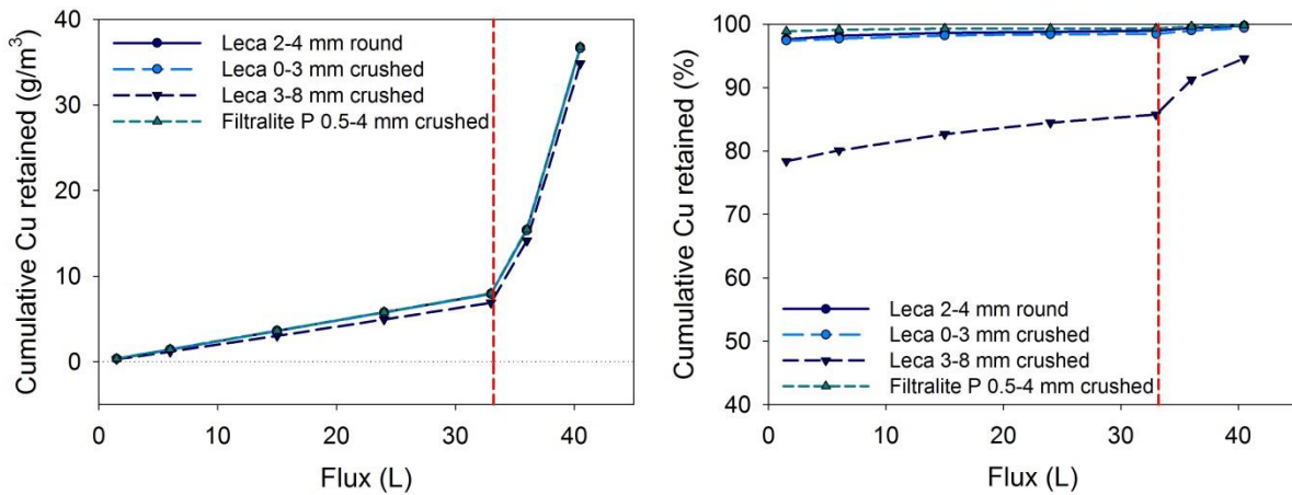
Figure 26. Cumulative copper (Cu) retention by Leca and Filtralite® products in flow-through column testing, expressed in \text{g/m}^3 (left) and as per cent of total (right).
