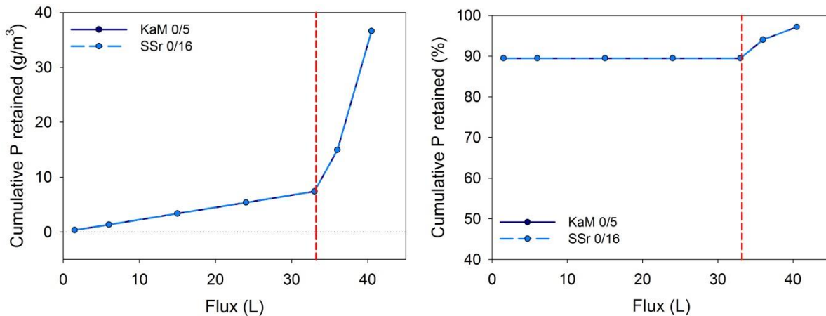
Figure 22. Cumulative phosphorus (P) retention by aggregate filter materials in flow-through column testing, expressed in g/m 3 (left) and as per cent of total (right).
