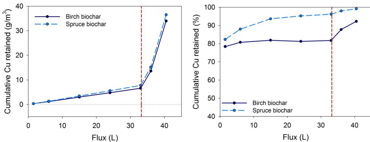
Figure 40. Cumulative copper (Cu) retention by biochar filter materials in flow-through column testing, expressed in \text{g}/\text{m}^3 (left) and as per cent of total (right).
