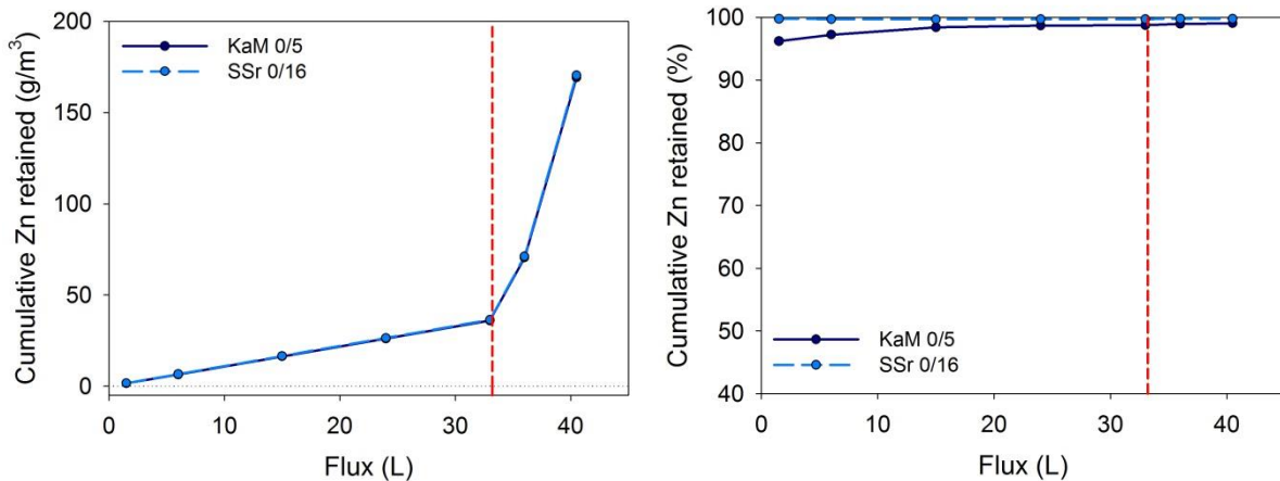
Figure 21. Cumulative zinc (Zn) retention by aggregate filter materials in flow-through column testing, expressed in g/m 3 (left) and as per cent of total (right).
