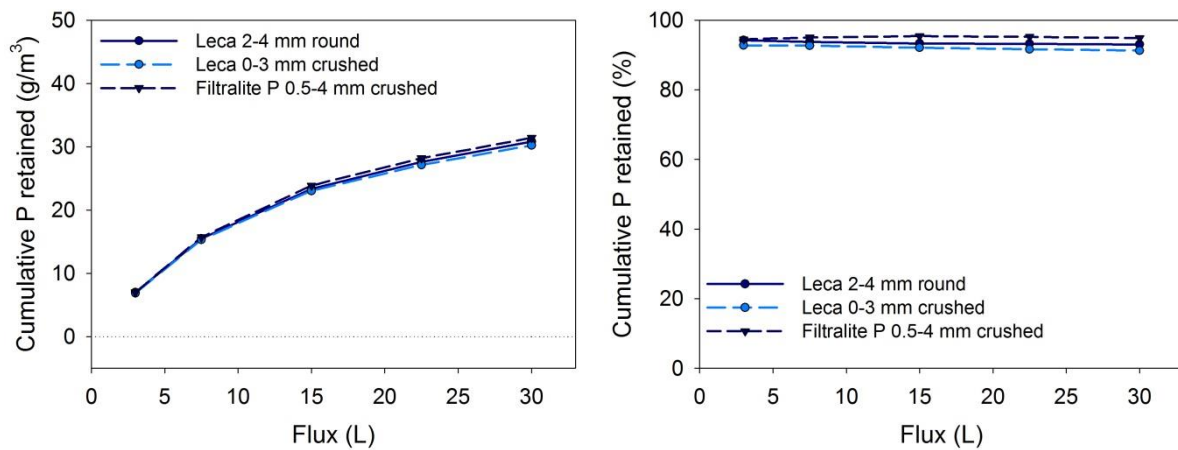
Figure 57. Cumulative phosphorus (P) retention by Leca and Filtralite ® products in column experiment using 10X concentrated synthetic stormwater, expressed in g/m 3 (left) and as per cent of total (right).
