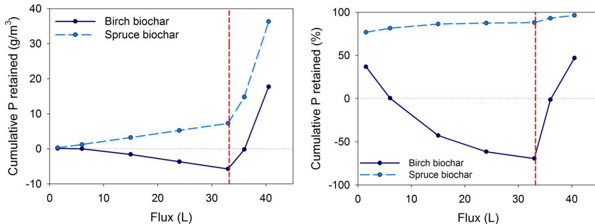
Figure 43. Cumulative phosphorus (P) retention by biochar filter materials in flow-through column testing, expressed in \text{g/m}^3 (left) and as per cent of total (right).
