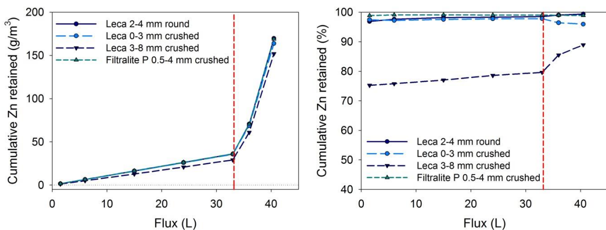
Figure 28. Cumulative zinc (Zn) retention by Leca and Filtralite® products in flow-through column testing, expressed in \text{g/m}^3 (left) and as per cent of total (right).
