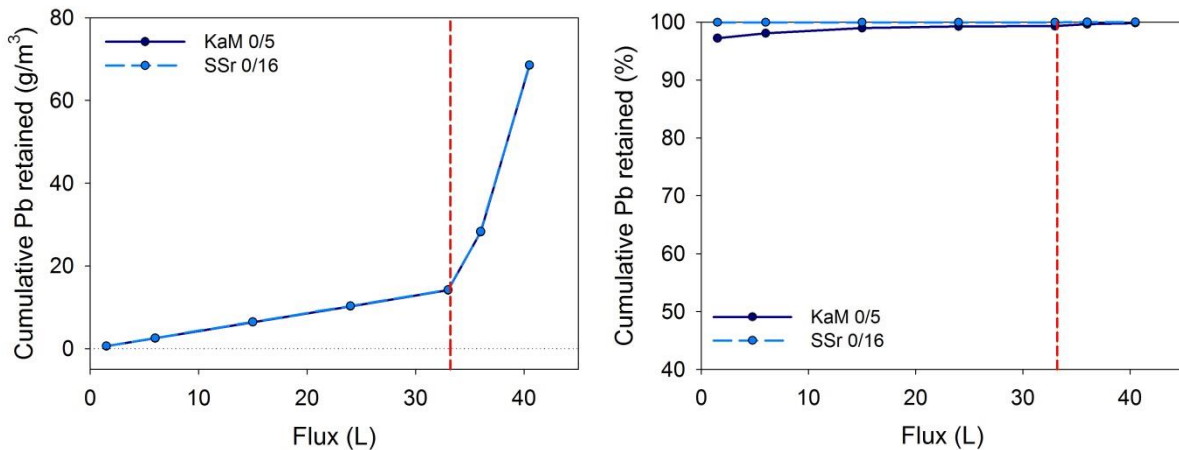
Figure 20. Cumulative lead (Pb) retention by aggregate materials in column testing, expressed in g/m 3 (left) and as per cent of total (right).
