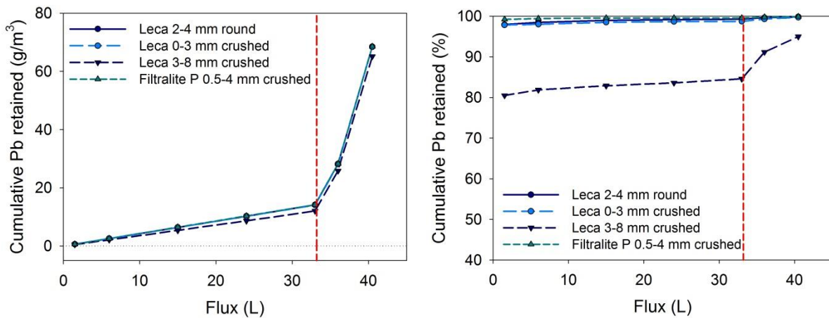
Figure 27. Cumulative lead (Pb) retention by Leca and Filtralite® products in flow-through column testing, expressed in \text{g/m}^3 (left) and as per cent of total (right).
