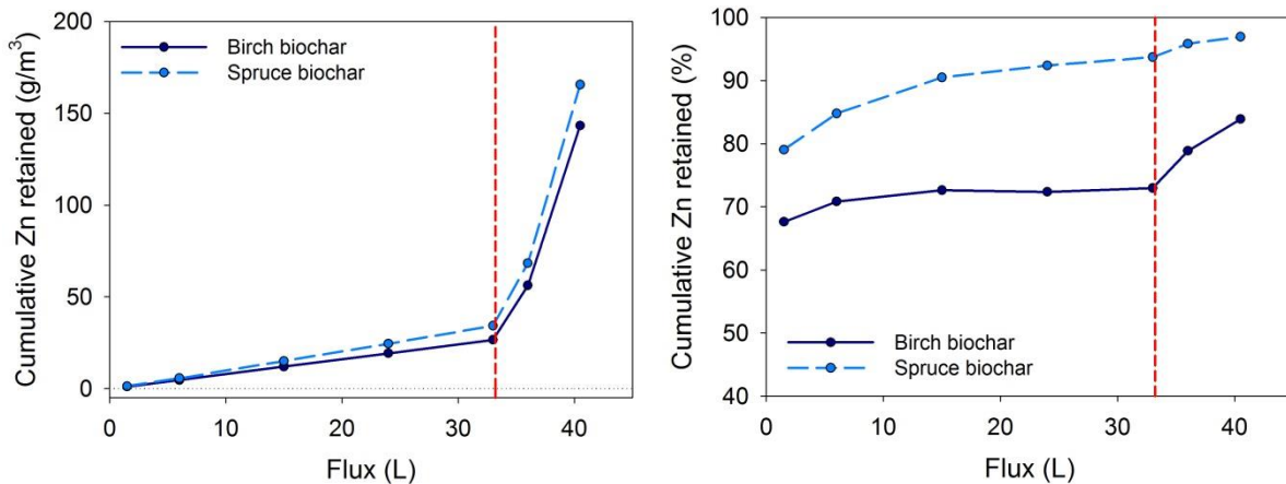
Figure 42. Cumulative zinc (Zn) retention by biochar filter materials in flow-through column testing, expressed in \text{g/m}^3 (left) and as per cent of total (right).
