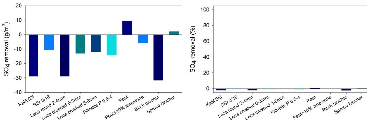
Figure 10. Overall sulfate ( \text{SO}_4^{2-} ) retention or release by filter materials in flow-through column testing, expressed in \text{g/m}^3 (left) and as per cent of total (right).
