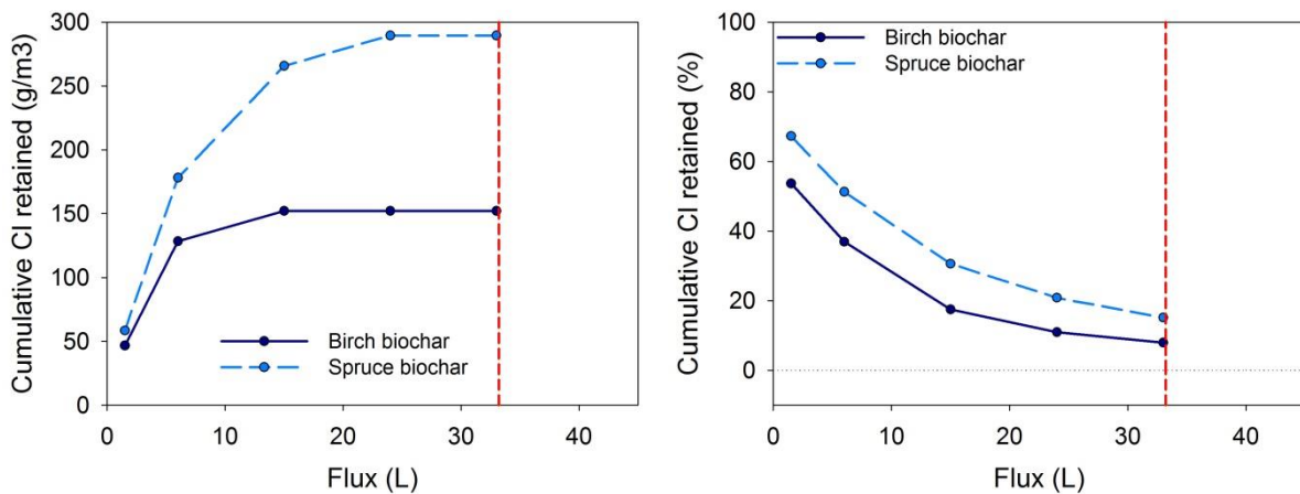
Figure 39. Cumulative chloride (Cl) retention by biochar filter materials in flow-through column testing, expressed in \text{g}/\text{m}^3 (left) and as per cent of total (right).
