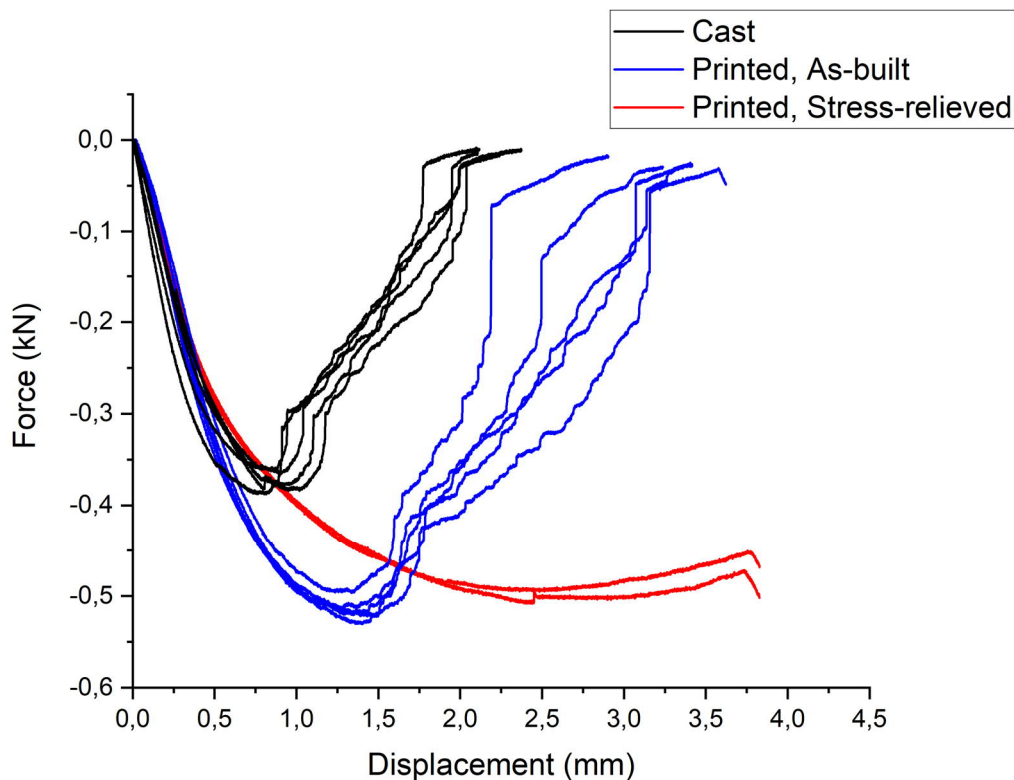
Figure 5. Force-Displacement curves obtained from the tests.
