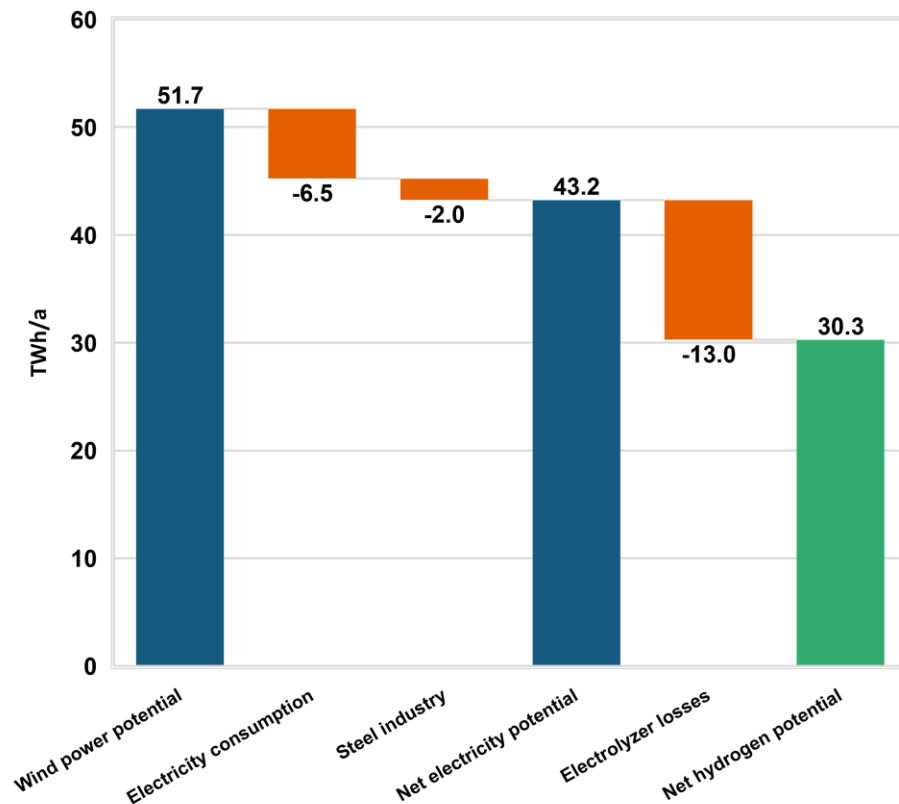
Figure 23. Net hydrogen potential in 2035 in Northern Ostrobothnia with half of the maximum projected wind power capacity.
