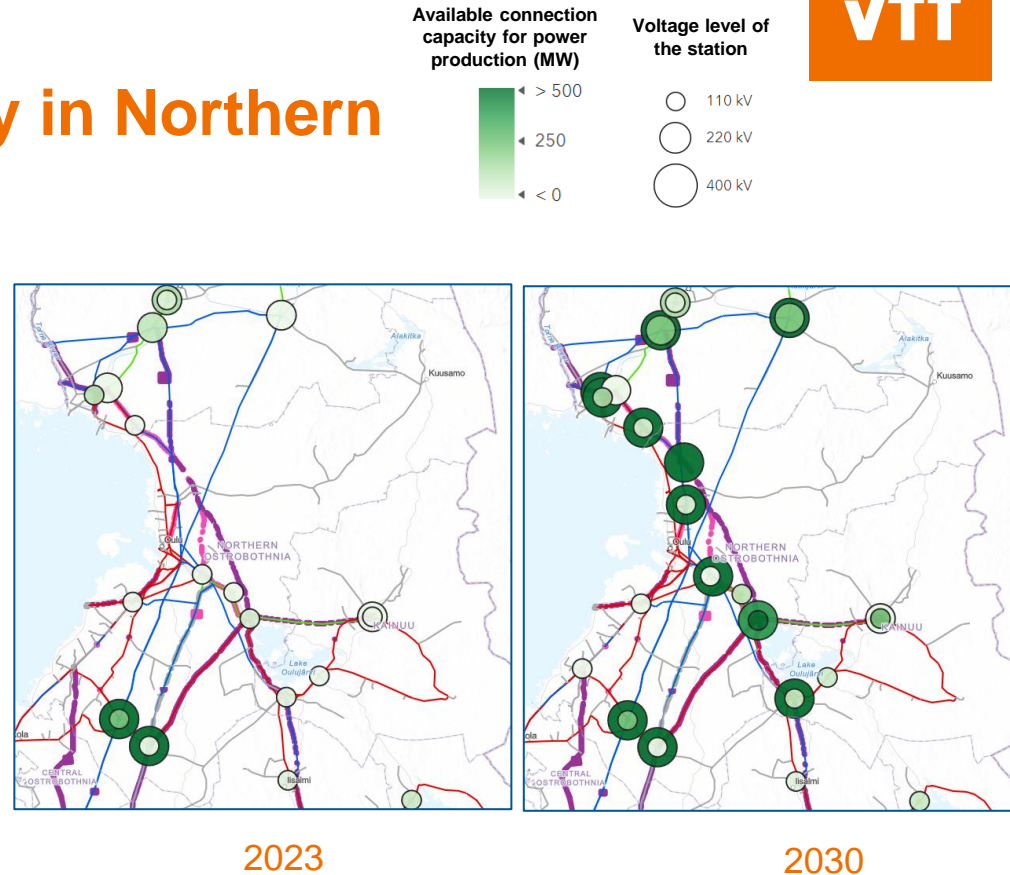
Figure 15: Available connection capacity to Fingrid's main grid in 2023 and 2030 [17].
