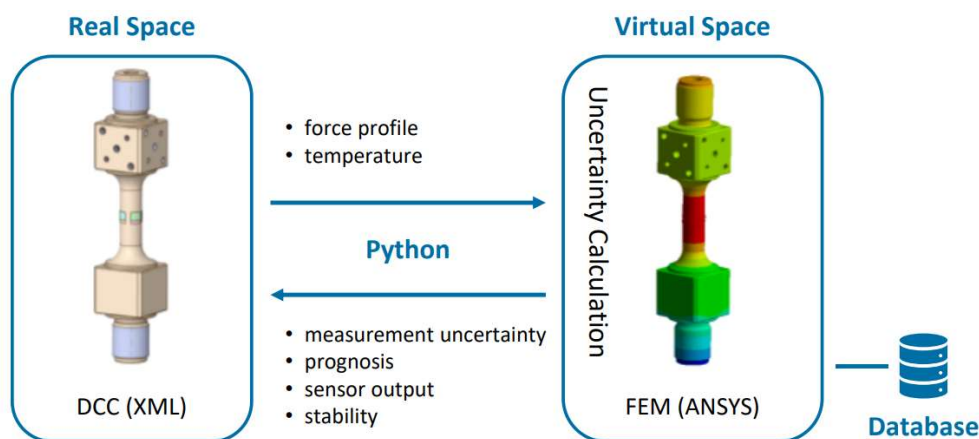
Figure 11 Concept of a Digital Metrological Twin of a force measurement device
