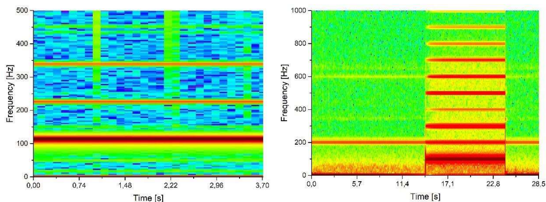
Figure 21 Impact of harmonics due to different sources on behaviour of a self-resonance and a hydraulic testing machine
