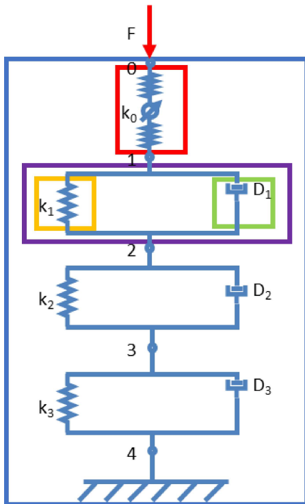
Figure 4 Extended generalized Kelvin Model: Red - Extended Hooke element; Yellow – Hooke element; Green – Newton Element; Purple – Kelvin -Voigt element
