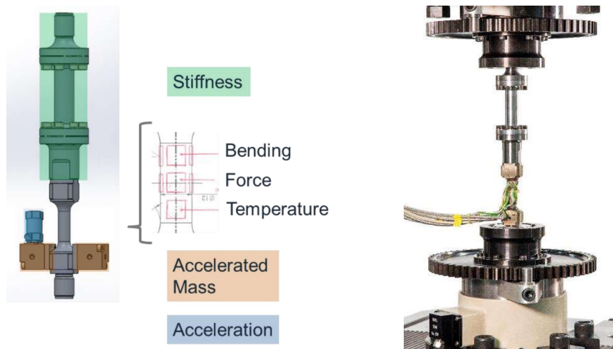
Figure 15: Set-up designed for dynamic machine calibration, with revised stiffness adapter; left: model; right: manufactured set-up applied to a 50 kN Rumul resonance testing system during approval
