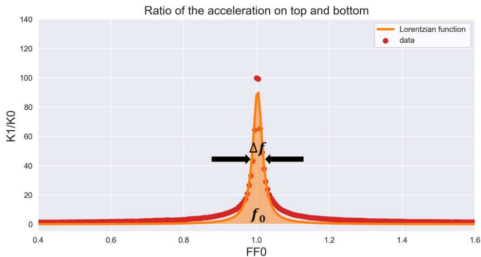
Figure 9 Resonance curve and Lorentzian function fit obtained after periodic chirp excitation to define model parameters
