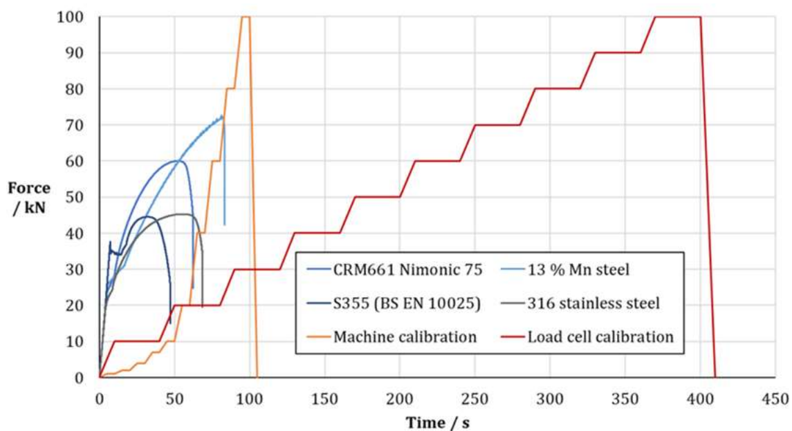
Figure 12 Diagram demonstrating force against time profiles for four different steel testpieces
