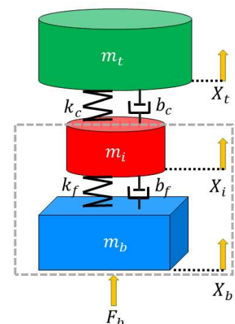
Figure 7 Schematic demonstration of the Kelvin-Voigt model
