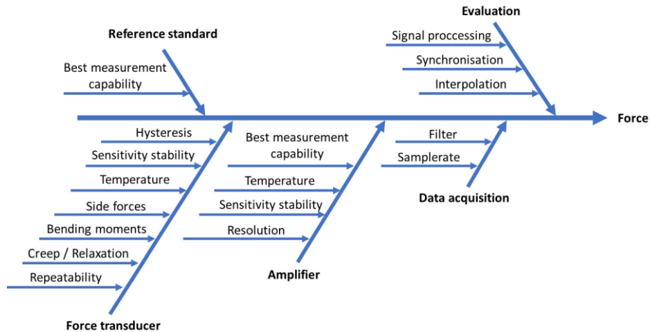
Figure 5 Ishikawa diagram of all influences on the indication of a force measuring device for continuous, quasi-static and static forces
