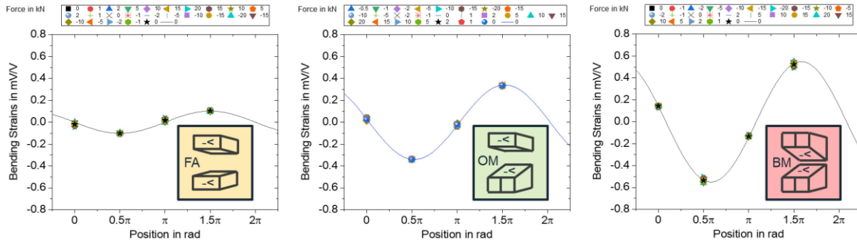
Figure 17: Calculated bending strains as a function of circumference under static loadings
