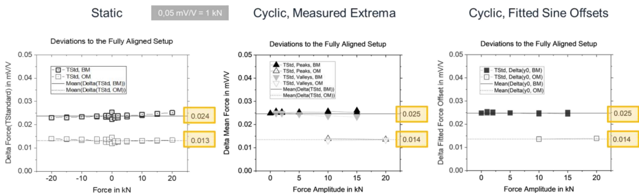
Figure 16: Force deviation due to bending strains, measurements at about 100 Hz on a 50 kN Rumul machine; left: static loadings; middle: cyclic loadings, extreme values evaluated, right: cyclic loadings, mean force y_0 evaluated
