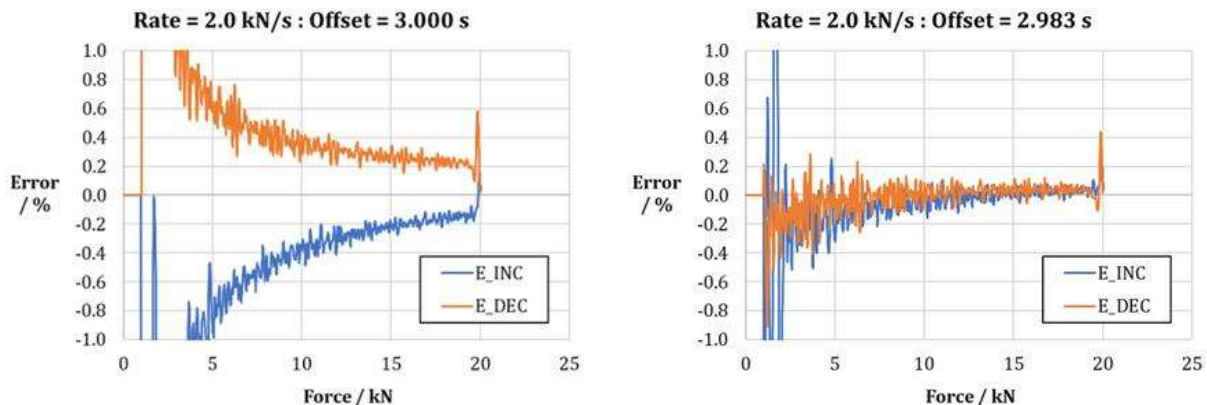
Figure 14 Diagram showing machine error against applied force using incremental and decremental errors
