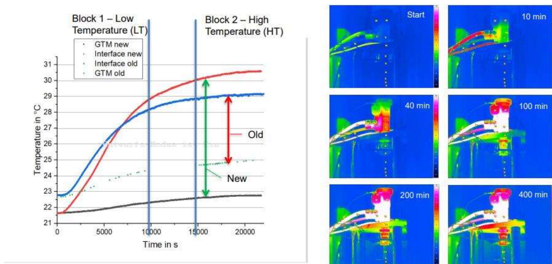
Figure 19 Left hand side shows the temperature increase during use of a servo-hydraulic machine and the influence of different adaptations between the two transducers. On the right hand side thermograph pictures for the identification of heat flows and resulting temperature gradients are shown.
