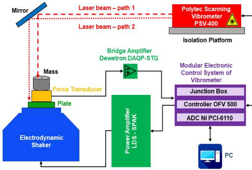
Figure 8 Dynamic force measurement set-up
