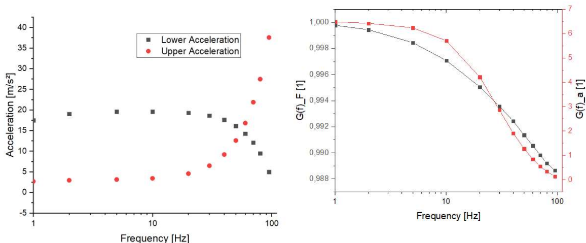
Figure 23 Left: Frequency response of the upper and lower acceleration measurement of the DUT transducer. Right: Transfer function of those accelerations and transfer function of the reference and DUT force measurements.
