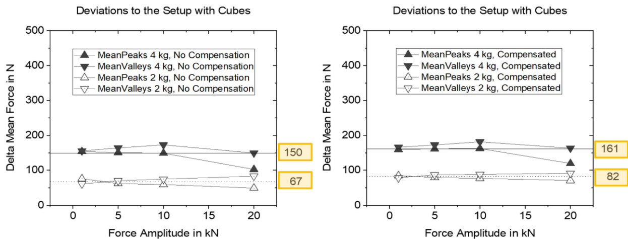
Figure 18: Force deviation due to additional masses, measurements at approx. 100 Hz on a 50 kN Rumul machine, where estimated masses to be compensated are: set-up with cubes (reference set-up): m \approx 13.7 kg, set-up named 2 kg: m \approx 18.7 kg, set-up named 4 kg: m \approx 20.7 kg; names of the set-ups, respectively the graphs in the charts are derived from mass elements excluding mounting elements; the differences between estimated masses and masses named are due to changes in mounting equipment needed to apply the masses; estimated masses are masses between sensing element of machine's force transducer and force plane of the dynamometer; left: mass not compensated by the software of the testing system, right: mass compensated by the software of the testing system, the value of computational compensation was set to 18.7 kg in the cases of 2 and 4 kg measurement series and to 13.7 kg in case of reference measurement with cubes.
