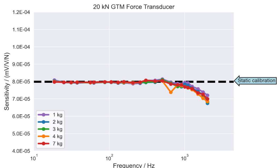
Figure 10 Dynamic sensitivity of 20kN GTM force transducers
