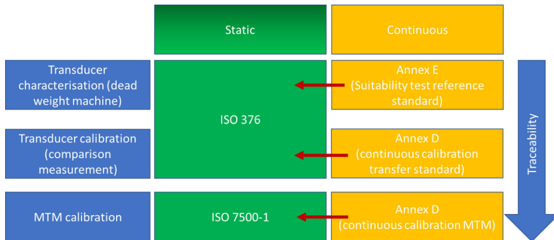
Figure 20 Proposed implementation of the new developed continuous calibration into the existing static normative traceability chain
