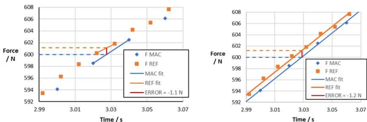
Figure 13 Examples of various interpolation approaches of measured data and resulting errors
