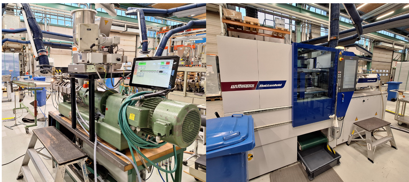
Figure 15. Compounder used for biocomposite compounding (left) and injection-moulding machine (right).
