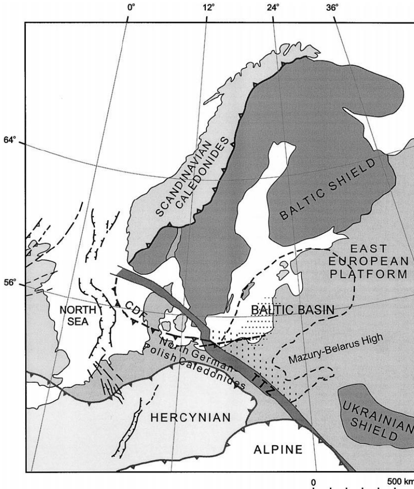
Figure 4. Major Tectonic structures and orogenic belts surrounding the Baltic Basin (Poprawa et al., 1999). 2
