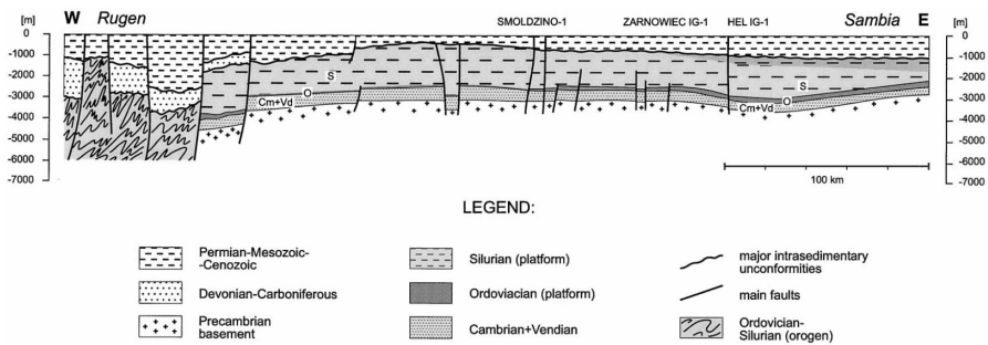
Figure 7. Sambia-Rugen cross section through the central western part of the Baltic Basin and the Caledonides (Poprawa et al., 1999). 3
