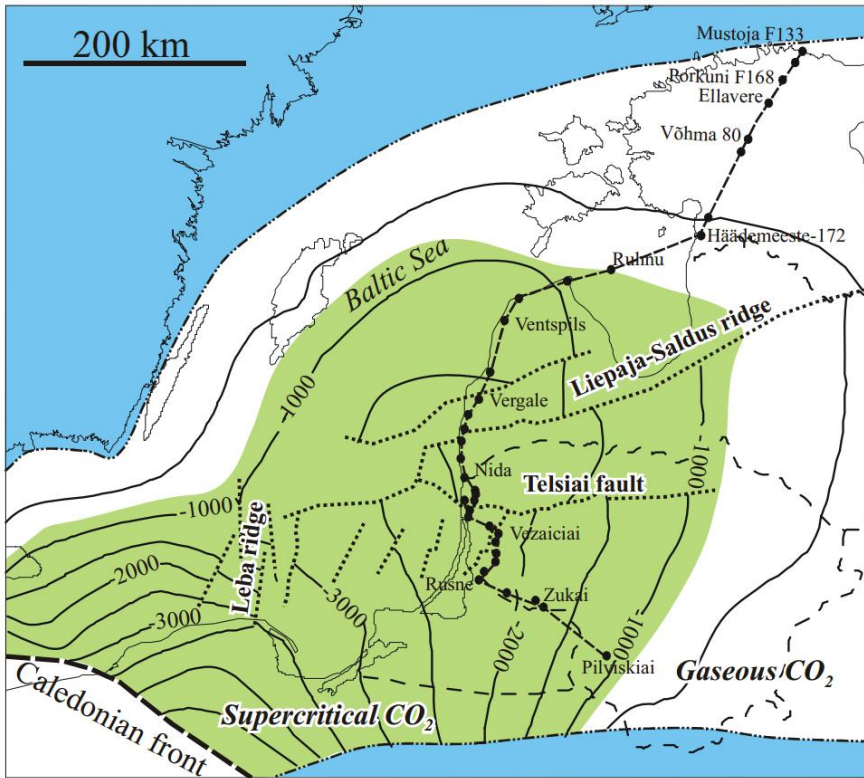
Figure 8. Depth of top of the Cambrian aquifer. 4
