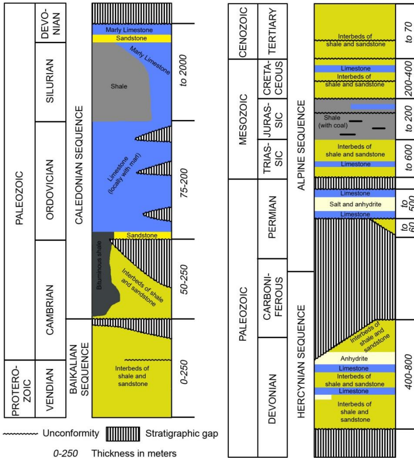
Figure 5. Stratigraphic Column of the Baltic Sea Basin showing the main depositional sequences (adapted from Ulmishek, 1990).
