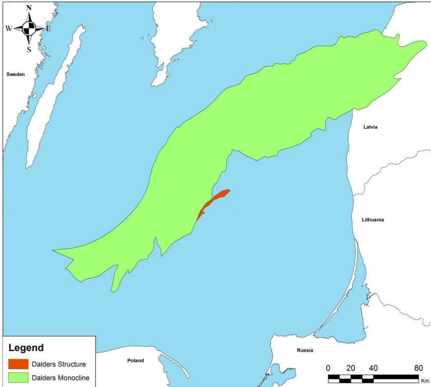
Figure 3. Location of the Dalders Structure and the Dalders Monocline.
