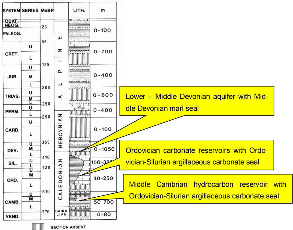
Figure 2. Geological section of the sedimentary basins in the Baltic Sea area (Brangulis et al., 1993).
