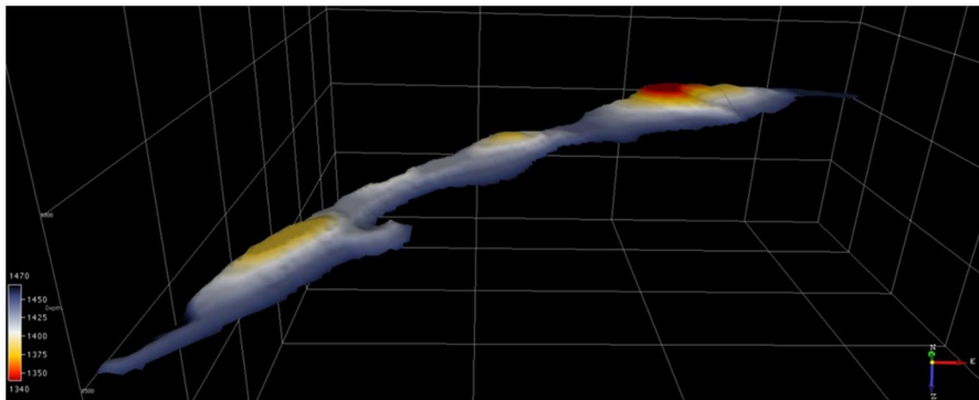
Figure 11. Top Cambrian layers of the Dalders structure.
