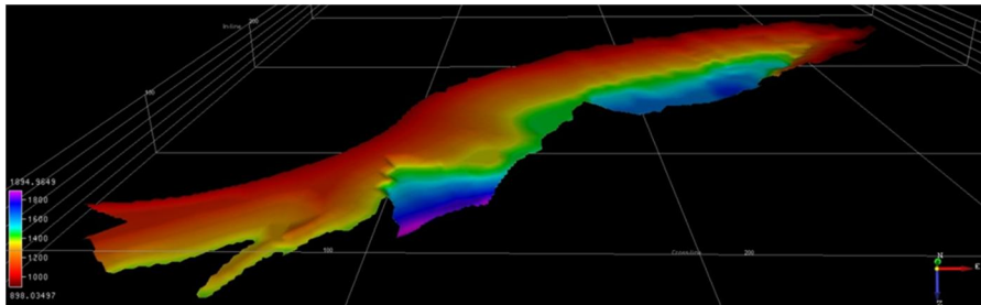
Figure 10. Top Cambrian layers of the Dalders Monocline.
