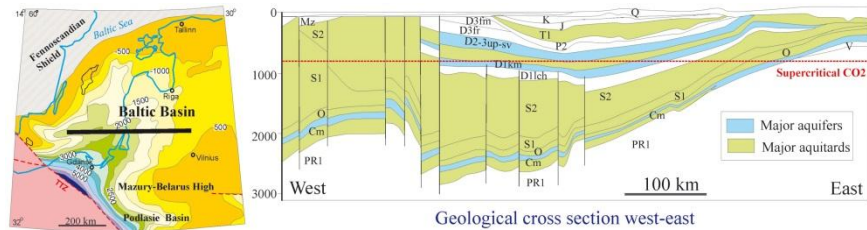
Depths of base of the Baltic Basin
