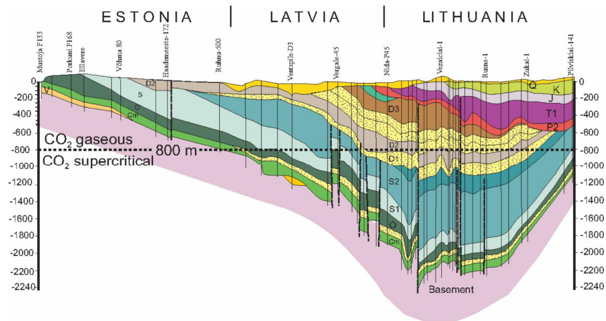
Figure 9. Geological cross section across Estonia, Latvia, and Lithuania (Shogenova et al., 2009b). 5
