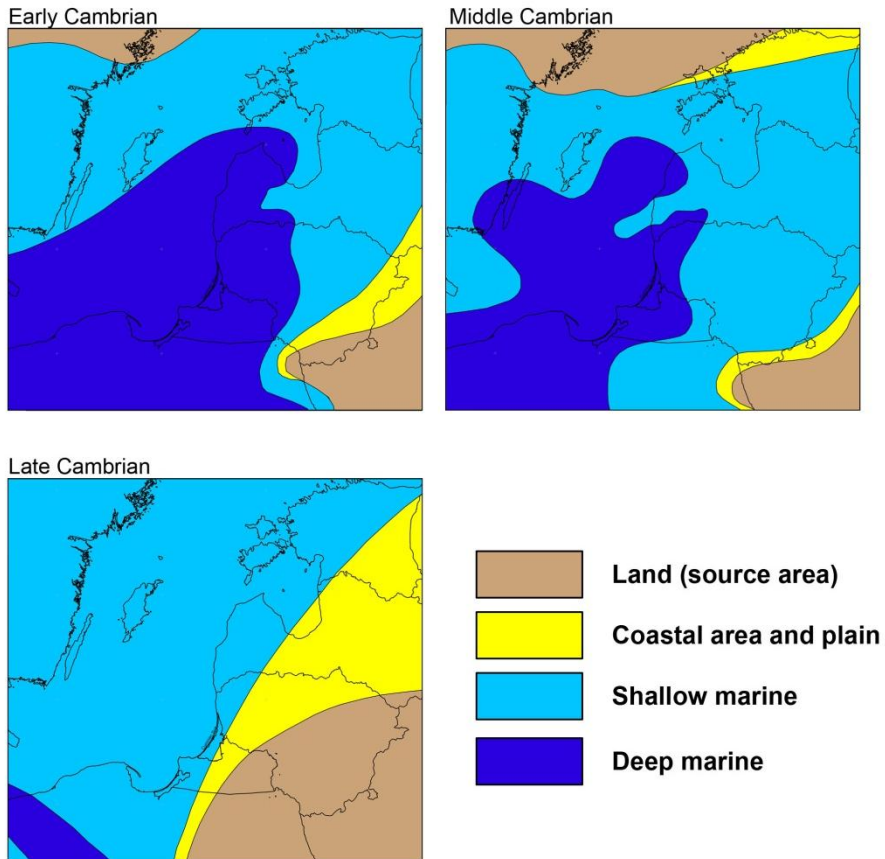
Figure 6. Reconstruction of the Cambrian paleoenvironment, separated into Early, Middle and Late Cambrian (after GSL, 1997).
