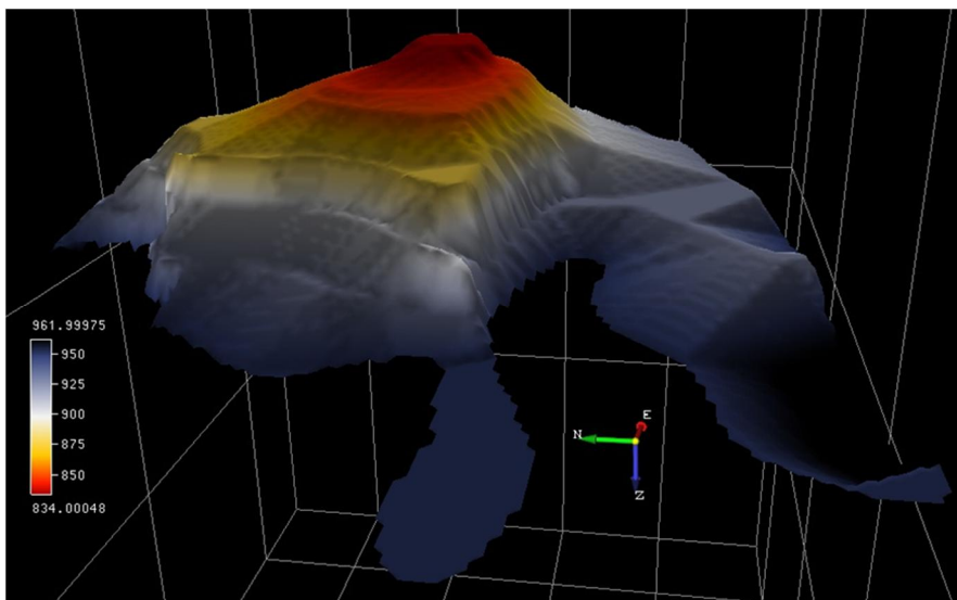
Figure 12. Top Cambrian layers of the E6 structure.
