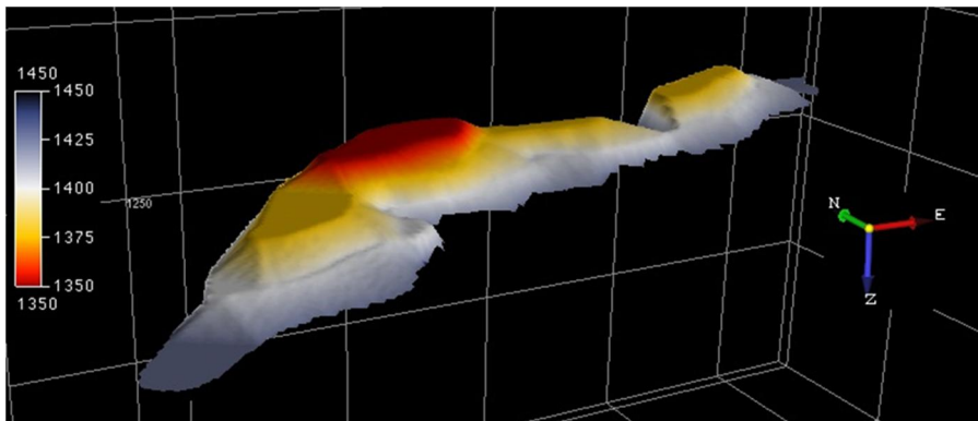
Figure 13. Top Cambrian layers of the E7 structure.
