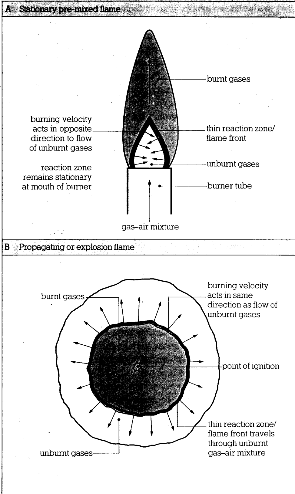
Figure 3.1. Stationary and propagating flames (Harris 1983).
