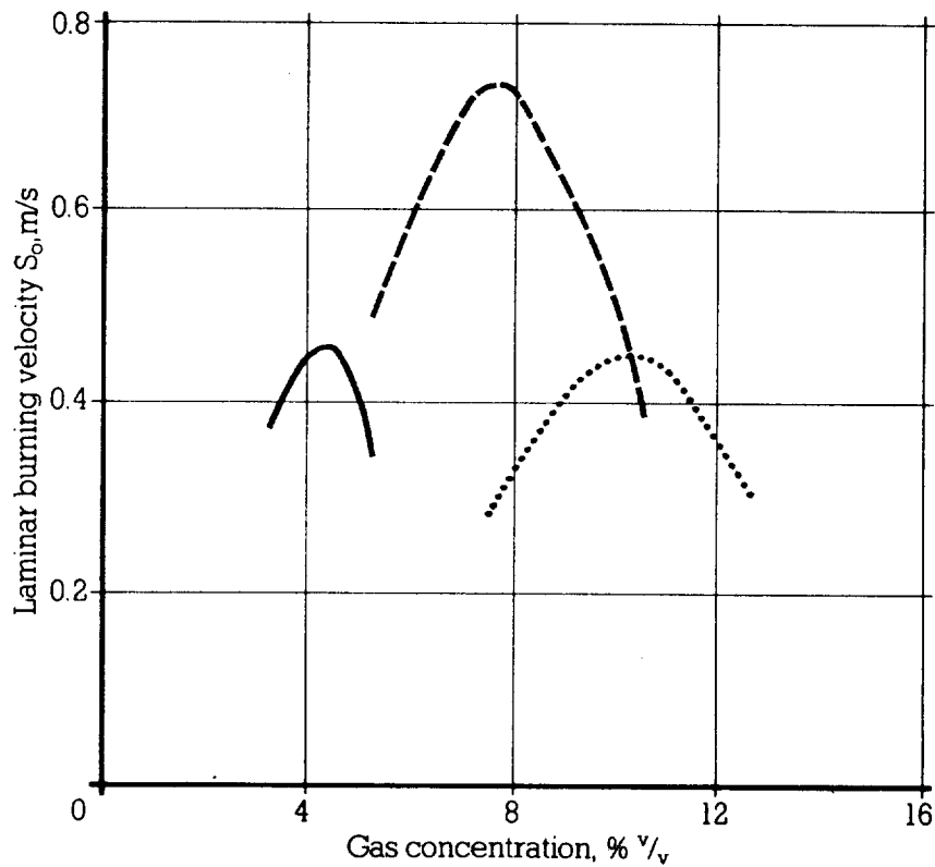
Figure 3.2. Effect of gas concentration on burning velocity. Solid line = propane, dashed line = ethylene, dotted line = methane (Harris 1983).
