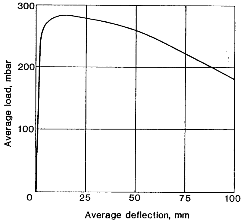
Figure 7.17. Example of a static load/deflection curve for a 114 mm thick brick wall of area 6.5 m 2 (Harris et al. 1985).
