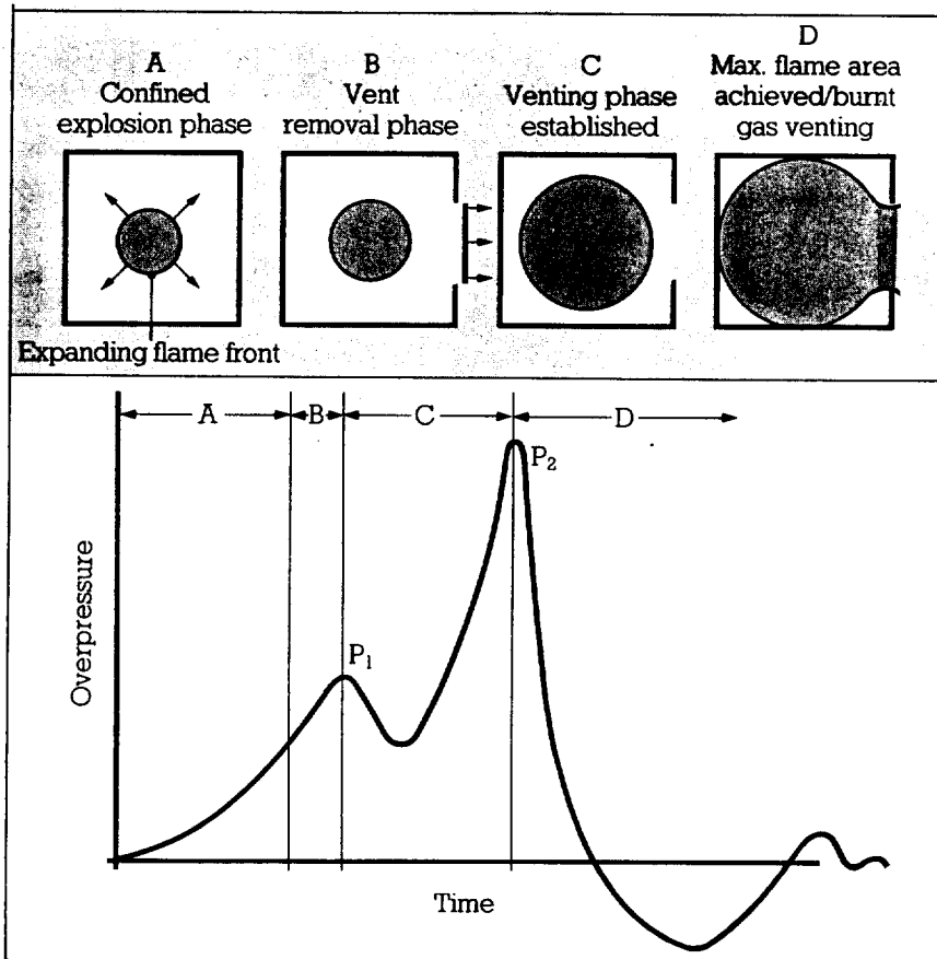
Figure 5.4. Origin of the first and second pressure peaks (Harris 1983).
