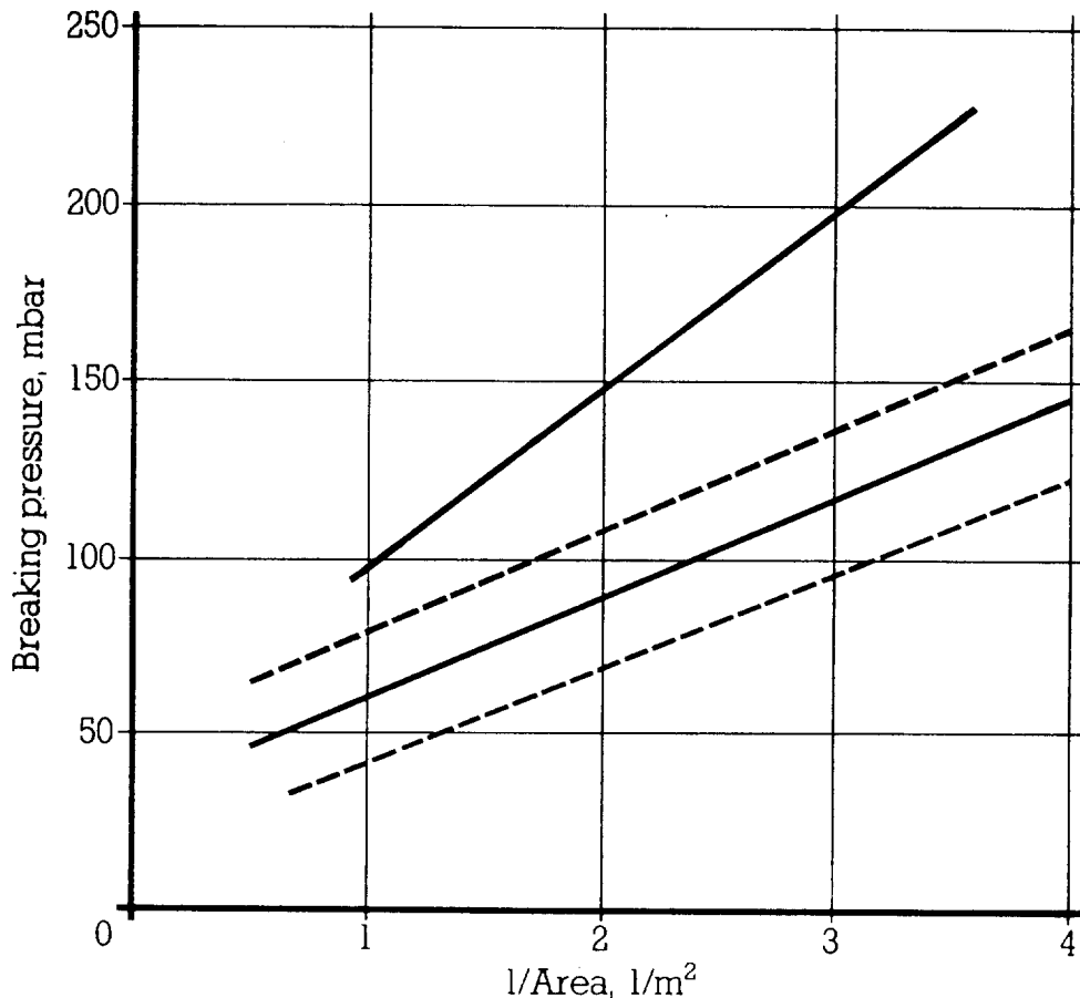
Figure 7.1. The breaking pressure of single-glazed glass windows as a function of pane area. The curves from top: 6.5 mm Georgian glass, 5 mm, 4 mm and 3 mm glass (Harris 1983).
