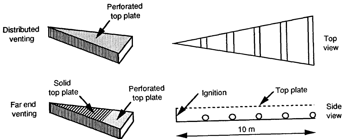
Figure 5.12. An wedge-shaped explosion vessel (Bjerketvedt et al. 1993).
