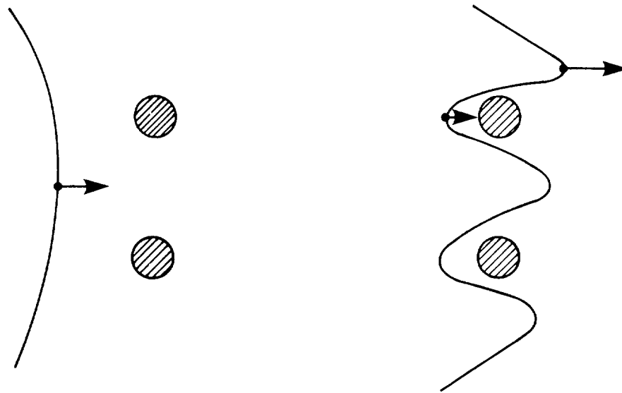
Figure 5.8. Flame folding caused by obstacles (British Gas 1992).
