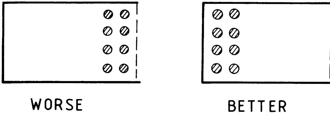
Figure 7.9. Preferable location of obstacles (Pappas 1984).
