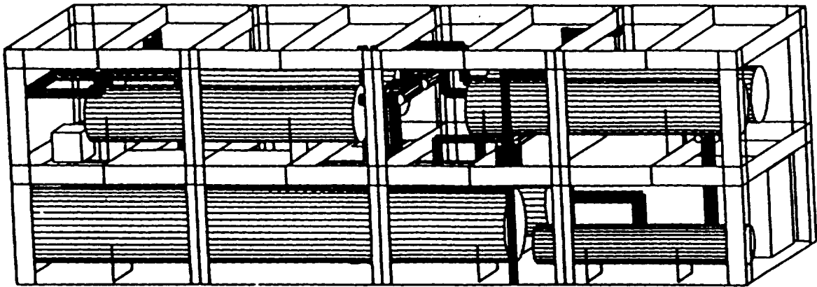
Figure 6.20. Internal layout of a 1:5 separator module (Hjertager et al. 1992).
