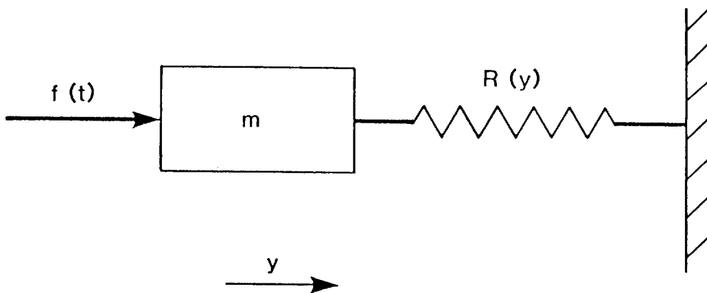
Figure 7.12. A simple forced spring and mass system (Harris et al. 1985).
