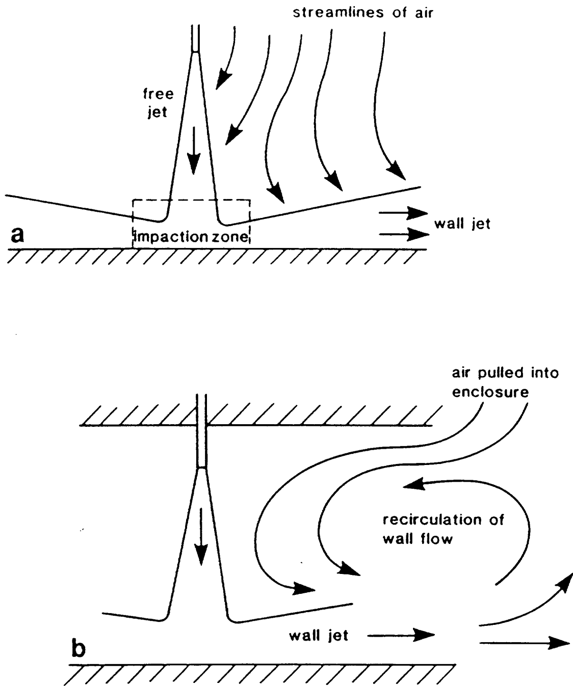
Figure 4.2. The effect of confinement in an impacting jet (Cleaver et al. 1994).
