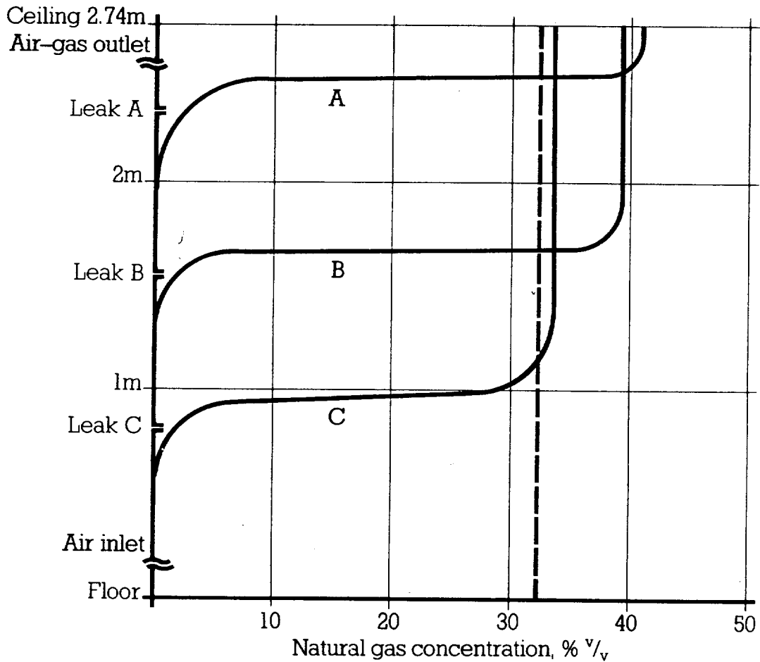
Figure 4.6. The effect of leak position on steady state concentration (Harris 1983).
