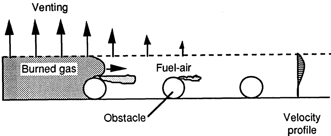
Figure 5.21. Early venting of hot combustion products will reduce turbulence generated by obstacles (Bjerketvedt et al. 1993).
