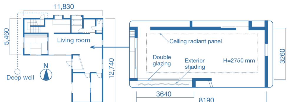
Figure 20. The house equipped with ceiling radiant cooling system using well water (Asada and Takeda 2002).
