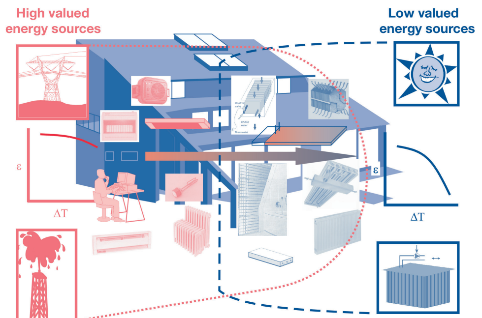
Figure 2. The transition from high valued energy sources to low valued energy sources requires appropriate heating and cooling systems in buildings. Heating and cooling systems that provide heating or cooling energy at a temperature close to room temperature (i.e., low exergy or LowEx systems) are a prerequisite for the efficient utilisation of low valued energy sources. On the other hand, the efficiency of high valued energy sources is less dependent on the heating and cooling systems in buildings.
