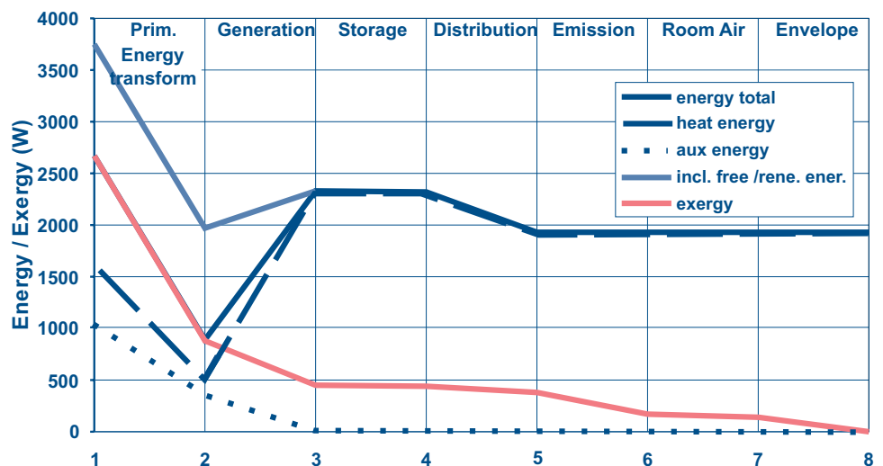
Figure 22. Exergy analysis of a floor heating system using a heat pump as energy generator.
