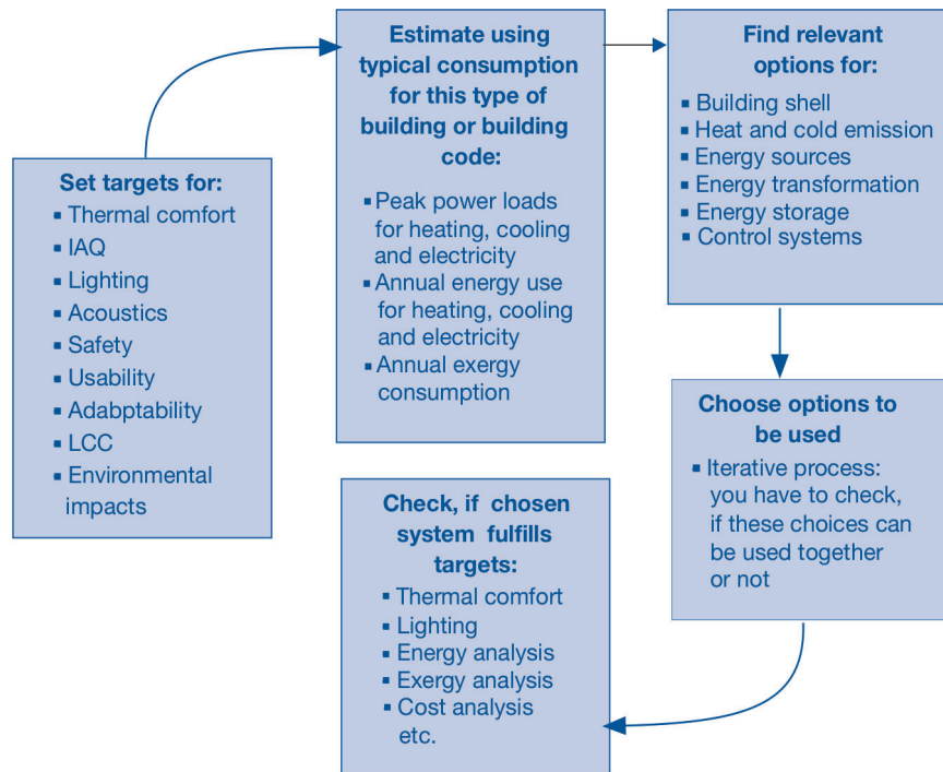
Figure 23. The design process of a building as a system.
