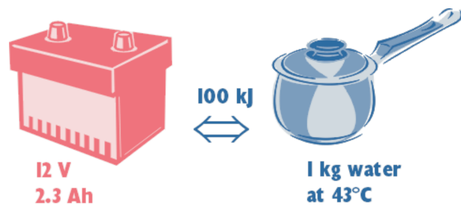
Figure 8. Both systems contain the same amount of energy but not the same amount of exergy.
