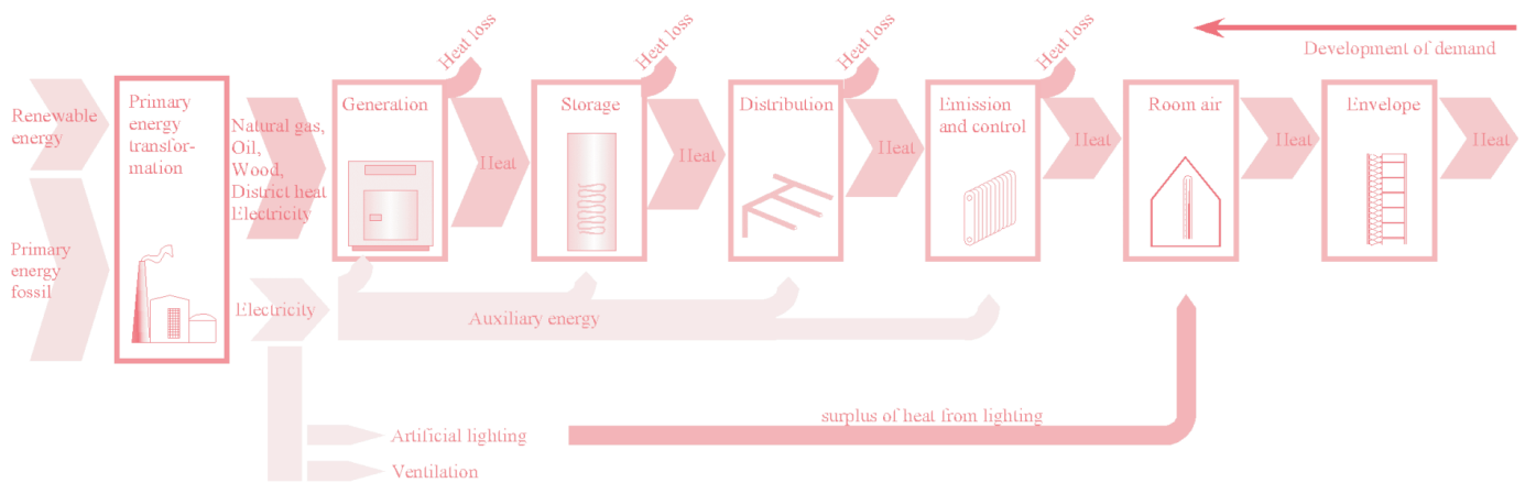
Figure 14. Energy utilisation in building services equipment, the modelling method for the pre-design tool. The energy flows are shown from source to sink, in accordance to DIN 4701-10, modified.
